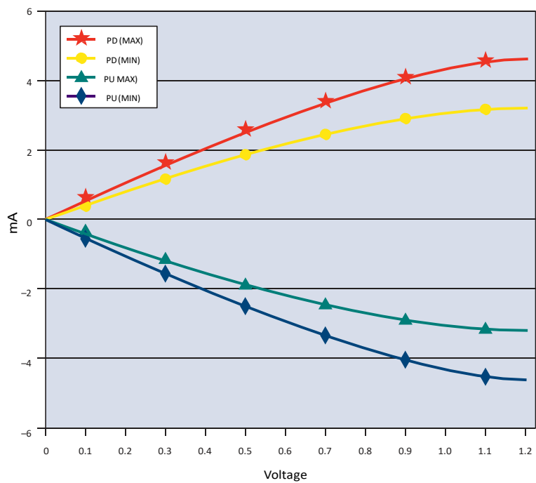
Output Impedance = 240 Ohms, I-V Curves After Calibration
