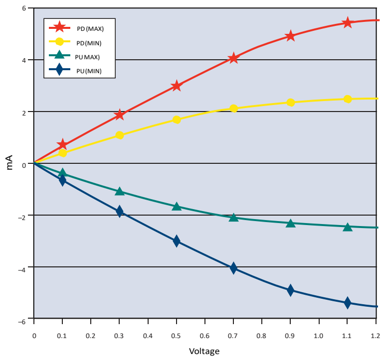
Output Impedance = 240 Ohms, I-V Curves After Calibration
