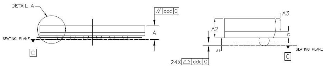
SIDE VIEW
