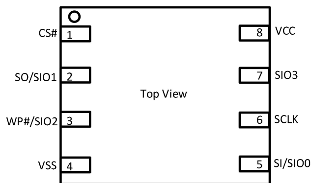
Figure1. Connection Diagram
