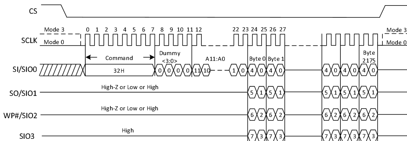
Figure19. Program Load x4 Sequence Diagram
