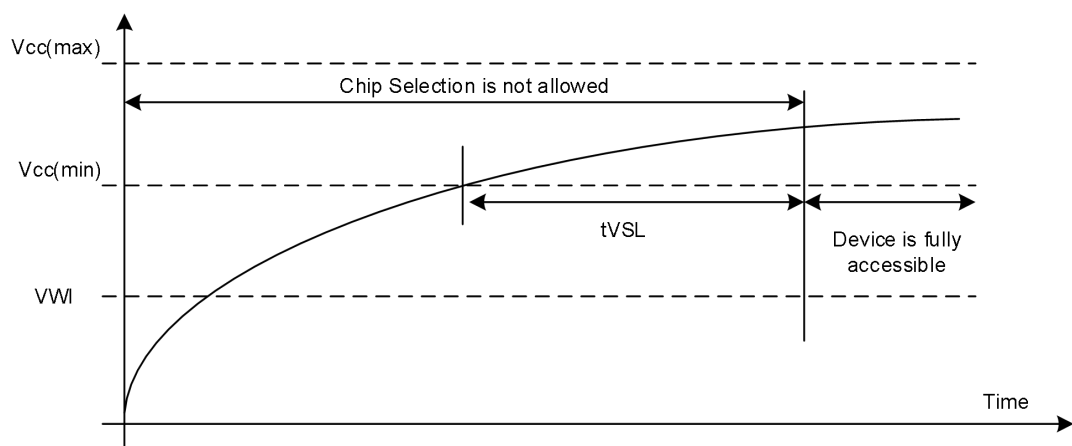
Figure26. Power-On Timing
