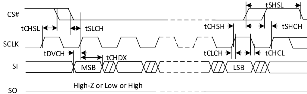
Serial Input Timing
