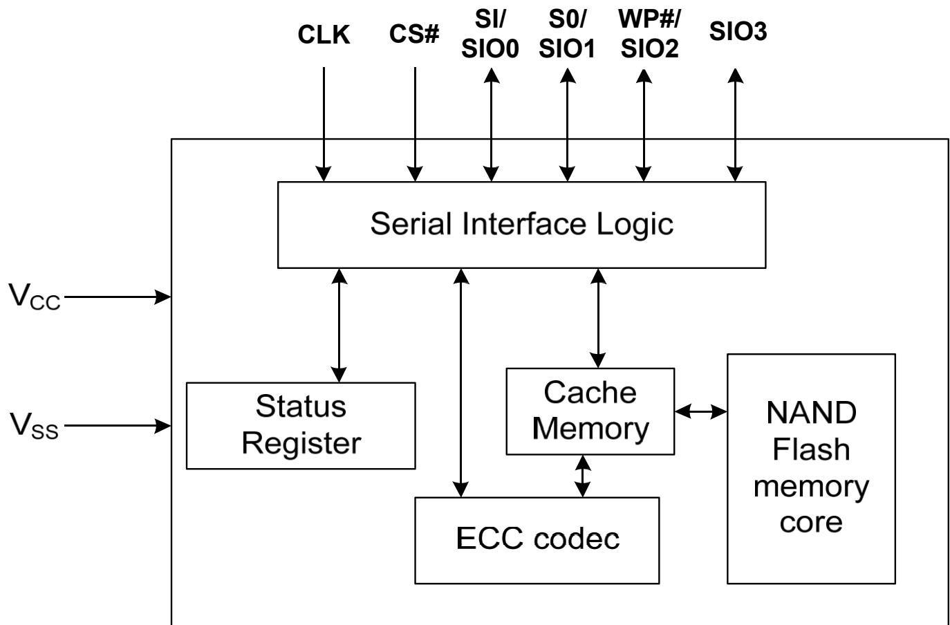
Figure2. Block Diagram
