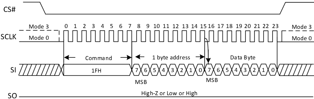
Figure8. Set Features Sequence Diagram
